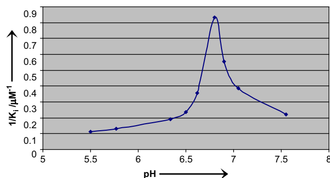
Chart 1. pH versus 1/K_i for 1 at 25 °C versus \beta -glucosidase from almonds.
