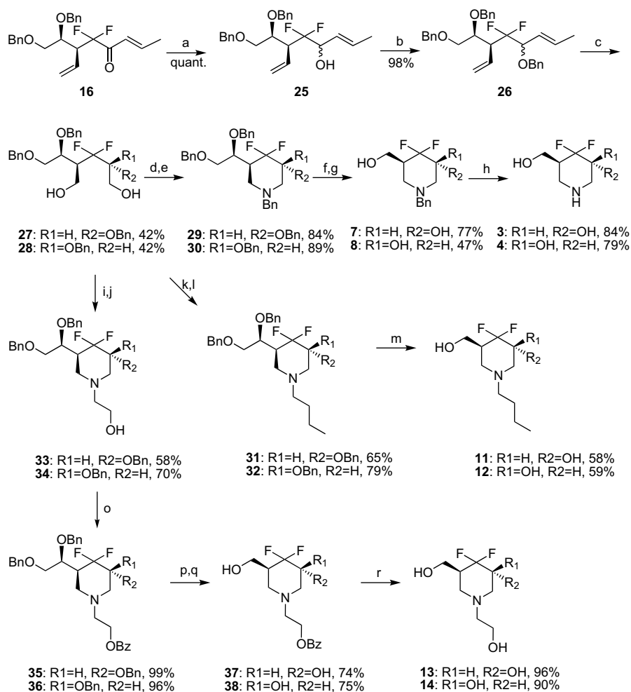
Scheme 2. Synthesis of 4,4-difluoroisofagomine analogues 3–4 , 7–8 , and 13–14 from compound 16 . Reagents and conditions: (a) NaBH 4 , CeCl 3 ·7H 2 O, MeOH, rt; (b) NaH, BnBr, TBAI, THF; (c) i. O 3 , CH 2 Cl 2 /MeOH (1:1), –78 °C; ii. NaBH 4 , –78 °C to rt; (d) i. MsCl, Et 3 N, DMAP, CH 2 Cl 2 ; ii. BnNH 2 , 80 °C; (e) i. BCl 3 (1 M) in heptane, CH 2 Cl 2 , 0 °C; ii. NaIO 4 , H 2 O, MeOH, rt; iii. NaBH 4 ; (f) 20% Pd(OH)/C, H 2 , MeOH, rt; (g) i. MsCl, Et 3 N, DMAP, CH 2 Cl 2 ; ii. H 2 NCH 2 CH 2 OH, 80 °C; (h) i. MsCl, Et 3 N, DMAP, CH 2 Cl 2 ; ii. n -BuNH 2 , reflux; (i) i. 20% Pd(OH)/C, H 2 , MeOH; ii. NaIO 4 , H 2 O, MeOH, rt; iii. NaBH 4 ; (j) BzCl, DMAP, Et 3 N, CH 2 Cl 2 ; (k) i. 10% Pd/C, H 2 , MeOH; ii. NaIO 4 , H 2 O, MeOH, rt; iii. NaBH 4 ; (l) NH 3 /MeOH.
