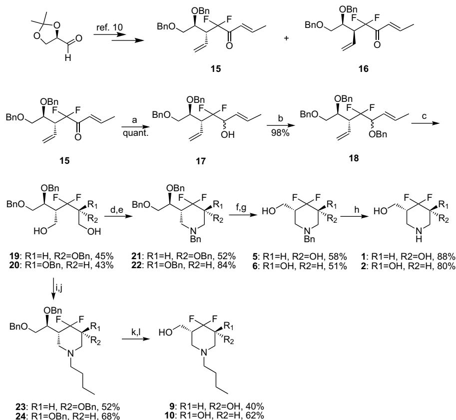
Scheme 1. Synthesis of 4-deoxy-4,4-difluoroisofagomine analogues 1–14 from compounds 15 and 16 . Reagents and conditions: (a) NaBH 4 , CeCl 3 ·7H 2 O, MeOH; (b) NaH, BnBr, TBAI, THF; (c) O 3 , CH 2 Cl 2 /MeOH (1:1), –78 °C, then NaBH 4 , –78 °C to rt; (d) MsCl, Et 3 N, DMAP, CH 2 Cl 2 ; (e) BnNH 2 , 80 °C; (f) i. BCl 3 (1 M in heptane), CH 2 Cl 2 , 0 °C; (g) NaIO 4 , H 2 O, MeOH, then NaBH 4 ; (h) 20% Pd(OH) 2 /C, H 2 , MeOH; (i) MsCl, Et 3 N, DMAP, CH 2 Cl 2 ; (j) n -BuNH 2 , reflux; (k) BCl 3 (1 M in heptane), CH 2 Cl 2 , 0 °C; (l) NaIO 4 , H 2 O, MeOH, then NaBH 4 .
