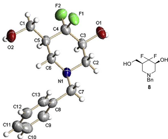
Figure 3. The X-ray crystallographic structure of compound 8 .
