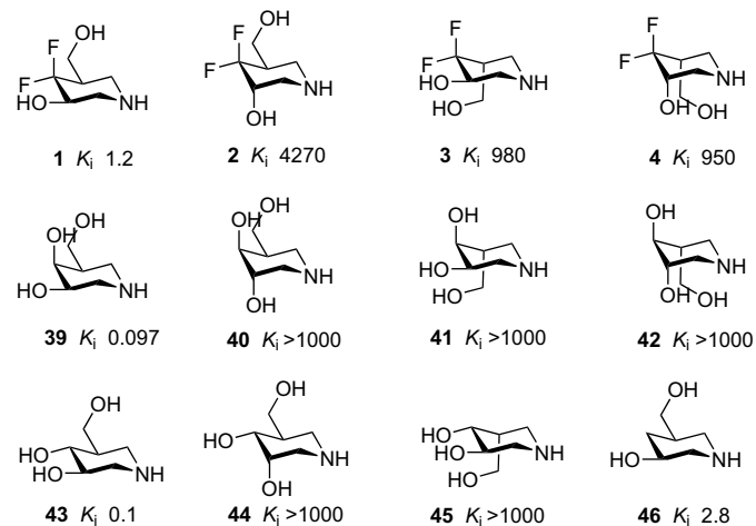
Figure 4. Comparison of the inhibition constants of 4-deoxy-4,4-difluoroisofagomine analogues 1–4 with their isofagomine analogues for \beta -glucosidase from almonds. Data for compounds 39–46 are taken from Refs. 7f and 14 . K_i in \mu M.
