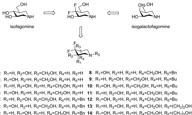
Figure 2. Rational design of 4-deoxy-4,4-difluoroisofagomine analogues 1–14.
